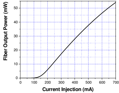
P-I Curve
